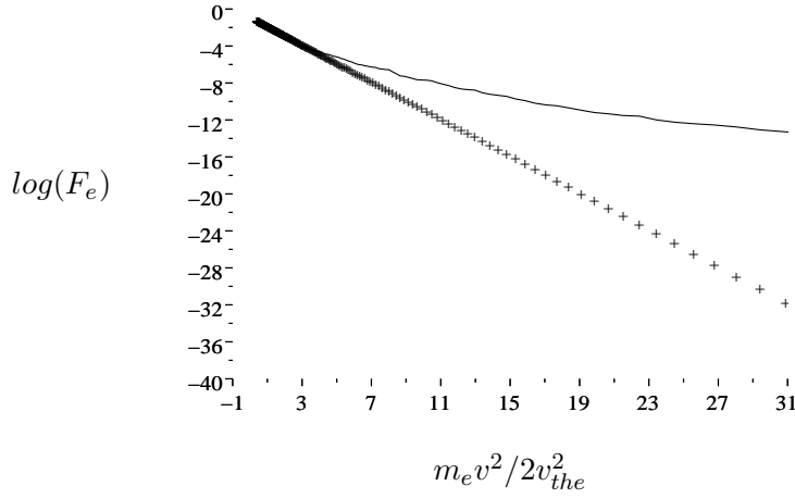
Figure 4: The solid line corresponds to the Log of the spatially averaged electron distribution versus the electron energy m_e v^2 / 2v_{the}^2 at the final time \omega_{pe} t = 16000 with |S|/\sqrt{4\pi n_0 T_e} = 8.10^{-3} and k_p \lambda_{De} = 0.09 and the dashed line corresponds to the initial electron distribution.
