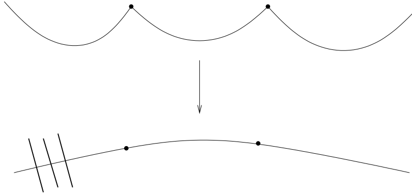
Figure 1: \mathcal{C}_{R'} \otimes_{R'} k \longrightarrow \mathbb{P}_k^1 with singularities and branch locus
