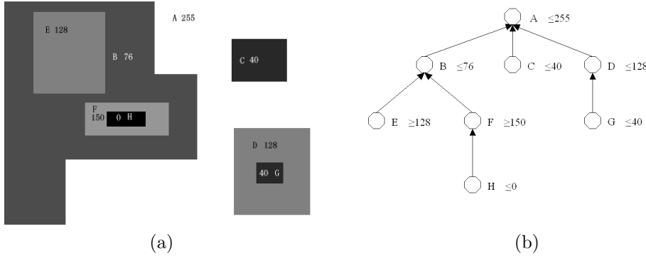
FIGURE 2.1. Example of FLST : (a) Synthetic image ; (b) Inclusion tree obtained with FLST.
