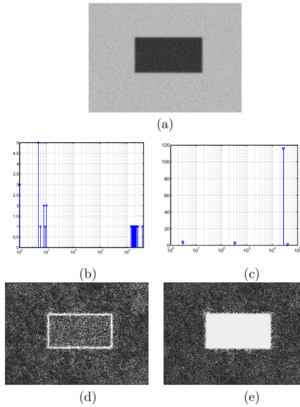
FIGURE 5.1. (a) Synthetic image of a rectangle degraded by blur and additive noise; (b) and (c) Values of the contrasts ((b): plain contrast, (c): cumulated contrast) of the shapes containing the central pixel as a function the area of the shape; (d) and (e) Corresponding area map ((d): using plain contrast, (e): using cumulated contrast) (for visualization, the gray level values correspond to the logarithm of the area).
