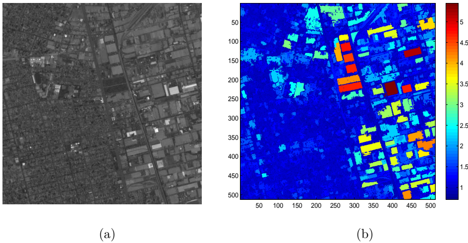
FIGURE 5.2. (a) Image of Los Angeles, SPOT5 (5m)©CNES; (b) Corresponding scale map. Notice the spatial accuracy of the method.
