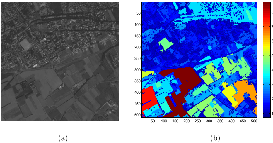
FIGURE 5.4. (a) Image of Marseille, SPOT5 (2.5m, 512 × 512)©CNES; (b) Corresponding scale map.
