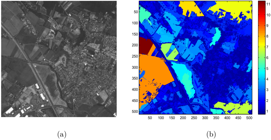
FIGURE 5.3. (a) Image of Toulouse, SPOT5 (5m)©CNES; (b) Corresponding scale map.
