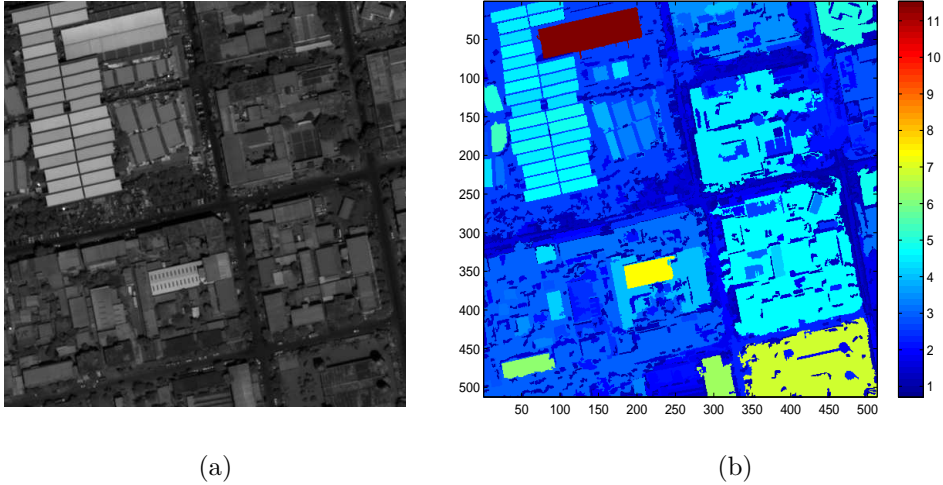
FIGURE 5.5. (a) Image of Ouagadougou, Quick-Bird (0.6m, 512 \times 512 )©CNES; (b) Corresponding scale map.
