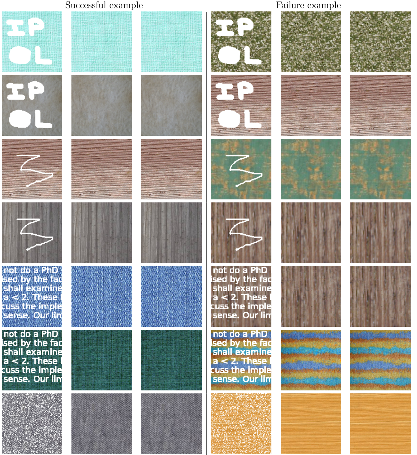
Figure 5: Examples of texture inpainting with k_{\max} = 100 and k_{\max} = 1000 . All images have size 128 \times 128 . Successful examples are presented in the left column while (relative) failure examples are presented in the right column (please zoom in for close inspection).
