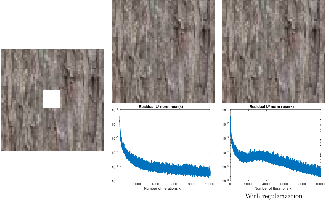
Figure 2: Convergence of the conjugate gradient method - \mathcal{C} = \Omega \setminus M . The first column contains the masked exemplar. The second and third columns contain the inpainting results without and with regularization, respectively. The inpainting results have been obtained with k_{\max} = 10000 iterations of the conjugate gradient on normal equations. Again, the residual norm decreases to 0 quite slowly. The regularization parameter \delta = 0.01 is not sufficient to improve the convergence. Still, the inpainting results are already satisfying, even without regularization. See the text for additional comments.
