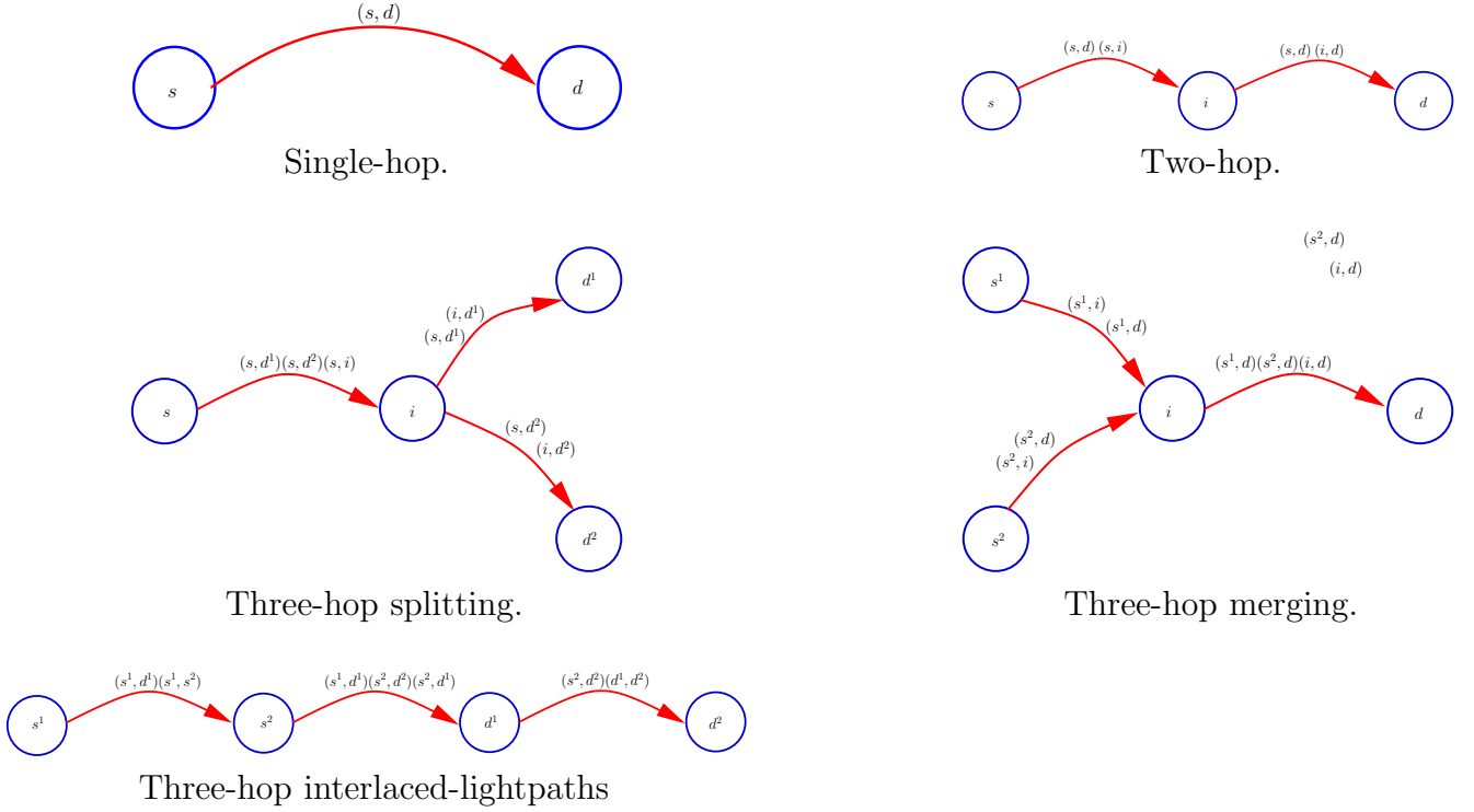
Figure 1: Optical hop configurations that define the supports of grooming patterns .
