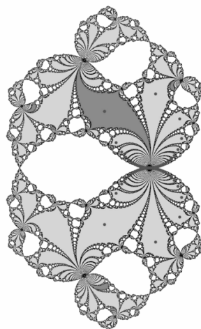
FIGURE 4. The set \mathcal{K}(\mathcal{L}_f) for f(z) = z + z^2 + 0.95z^3 .
