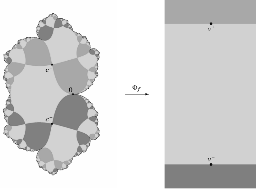
Fig. 6 Behavior of \Phi_f for f(z) := z + z^2 + 0.95z^3 . Right: three regions delimited by the horizontal lines passing through the critical values of \Phi_f . Left: the basin \mathcal{B}_f is tiled by the preimages of those three regions by \Phi_f .
