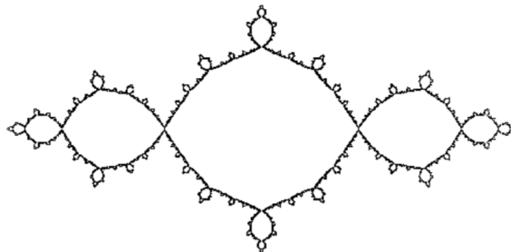
FIGURE 1. The Julia set of the quadratic polynomial f : \widehat{\mathbb{C}} \rightarrow \widehat{\mathbb{C}} defined by f(z) = z^2 - 1 .
