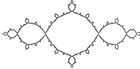
Fig. 1 The Julia set of the quadratic polynomial f : \widehat{\mathbb{C}} \rightarrow \widehat{\mathbb{C}} defined by f(z) = z^2 - 1 .
