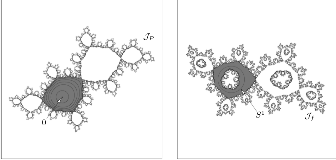
FIGURE 2. Left: the polynomial P : z \mapsto e^{i\pi(\sqrt{5}-1)z} + z^2 has a Siegel disk (colored grey). We have drawn the orbits of some points in the Siegel disk. Each orbit accumulates on a \mathbb{R} -analytic circle. Right: if t \in \mathbb{R}/\mathbb{Z} is chosen carefully enough, the rational map f(z) = e^{2i\pi t} z^2(z-4)/(1-4z) has a Herman ring. It leaves the circle S^1 invariant and is conjugate to an irrational rotation on S^1 . The picture is drawn for t = 0.61517321588\dots
