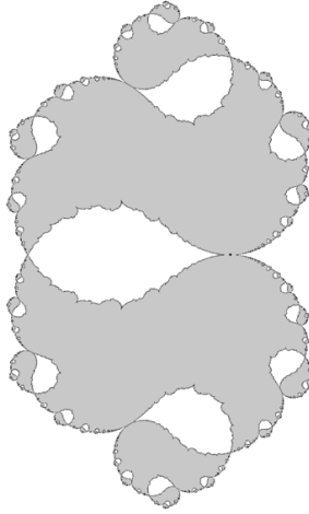
Fig. 7 Behavior of \mathcal{L}_f for f(z) := z + z^2 + 0.95z^3 .
