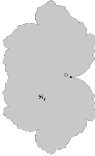
Fig. 5 For the cubic polynomial f(z) = z + z^2 + 0.95z^3 , the basin \mathcal{B}_f (grey) is the interior of the filled-in Julia set \mathcal{K}_f .
