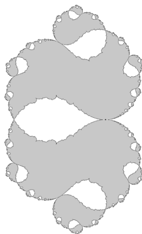
FIGURE 3. Behavior of \mathcal{L}_f for f(z) := z + z^2 + 0.95z^3 .
