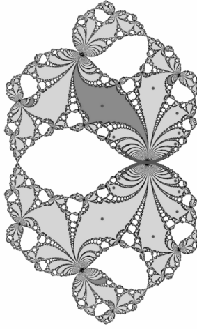
Fig. 8 The set \mathcal{K}(\mathcal{L}_f) for f(z) = z + z^2 + 0.95z^3 .
