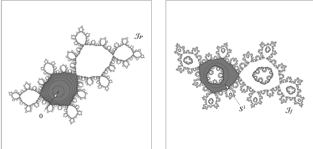
Fig. 4 Left: the polynomial P : z \mapsto e^{i\pi(\sqrt{5}-1)}z + z^2 has a Siegel disk (colored grey). We have drawn the orbits of some points in the Siegel disk. Each orbit accumulates on a \mathbb{R} -analytic circle. Right: if t \in \mathbb{R}/\mathbb{Z} is chosen carefully enough, the rational map f(z) = e^{2i\pi t} z^2(z-4)/(1-4z) has a Herman ring. It leaves the circle S^1 invariant and is conjugate to an irrational rotation on S^1 . The picture is drawn for t = 0.61517321588 \dots
