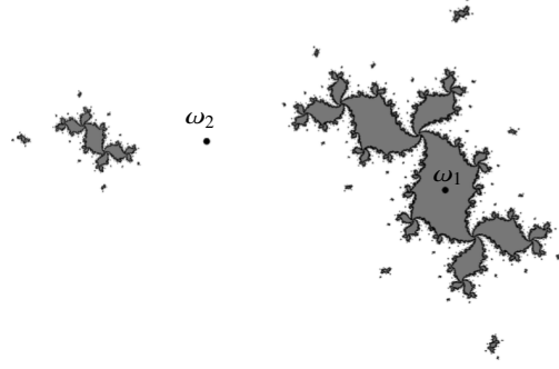
Fig. 3 The filled-in Julia set of a cubic polynomial. The critical point \omega_1 is in \mathcal{K}_f . The other critical point \omega_2 is in the basin of infinity. The Julia set \mathcal{J}_f is not connected.
