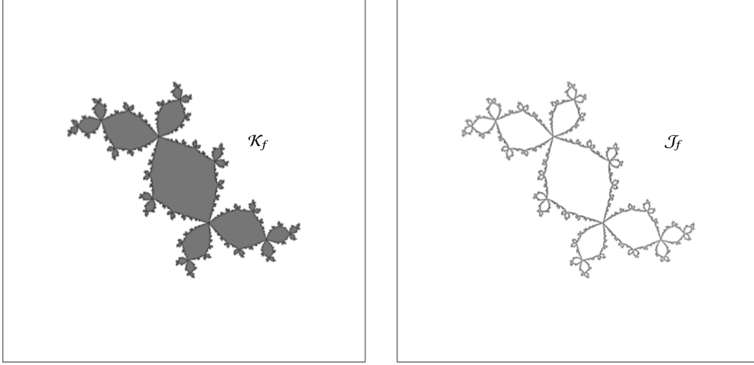
Fig. 2 Left: the filled-in Julia set of a quadratic polynomial. It is known as the Douady Rabbit. Right: the Julia set for the same quadratic polynomial. It is the topological boundary of the filled-in Julia set.
