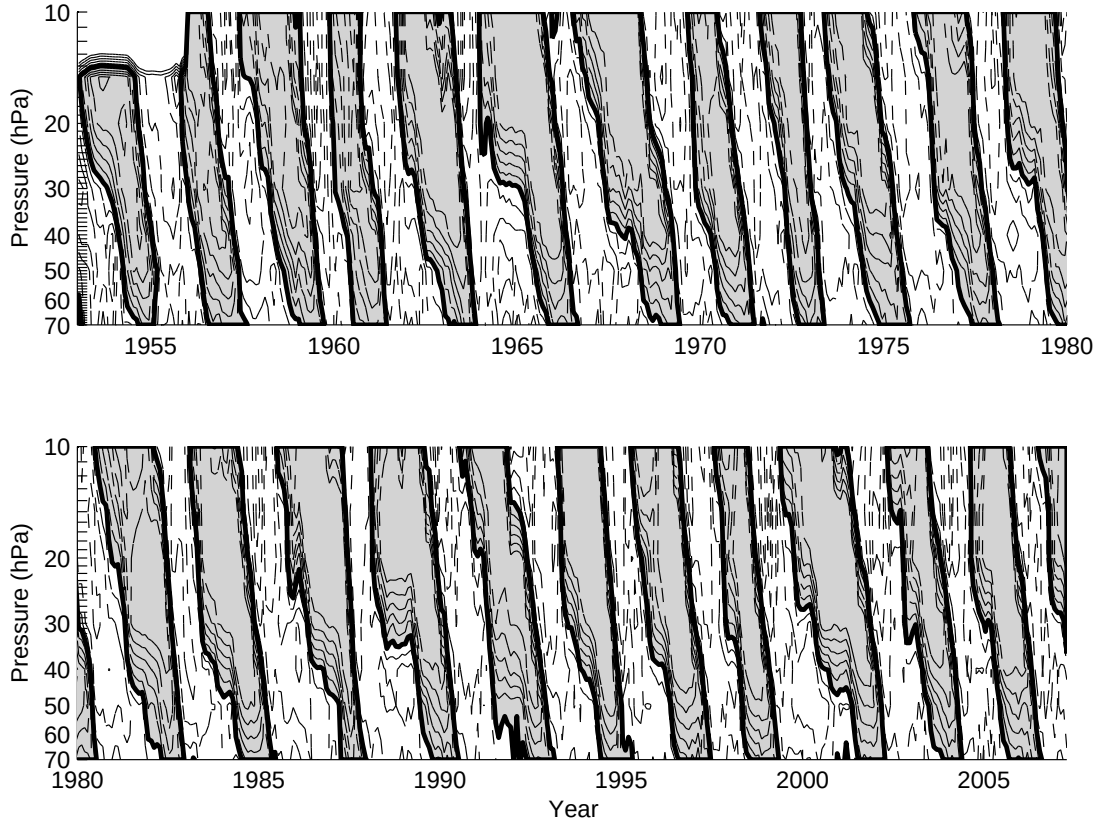
Figure 1. Time-height section of the FUB zonal wind. Easterlies are shown shaded.
