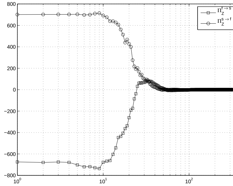
FIGURE 9. Cross fluxes of enstrophy ( k_{inj} \approx 20 ).
