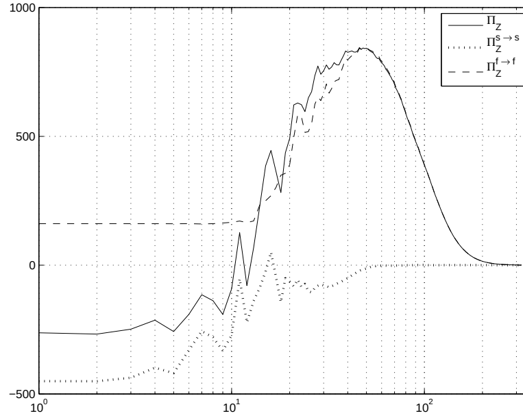
FIGURE 8. Enstrophy fluxes of the whole flow and of the separate structures ( k_{inj} \approx 20 ).
