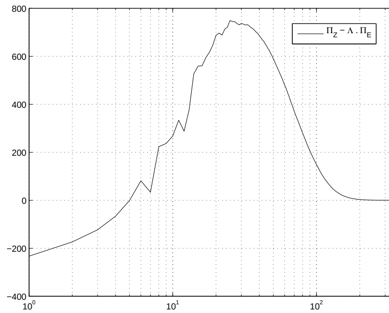
FIGURE 6. \Pi_Z - \Lambda \Pi_E allowing to verify the Danilov inequality.
