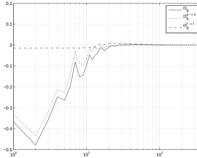
FIGURE 7. Energy fluxes of the whole flow and of the separate structures ( k_{inj} \approx 20 ).
