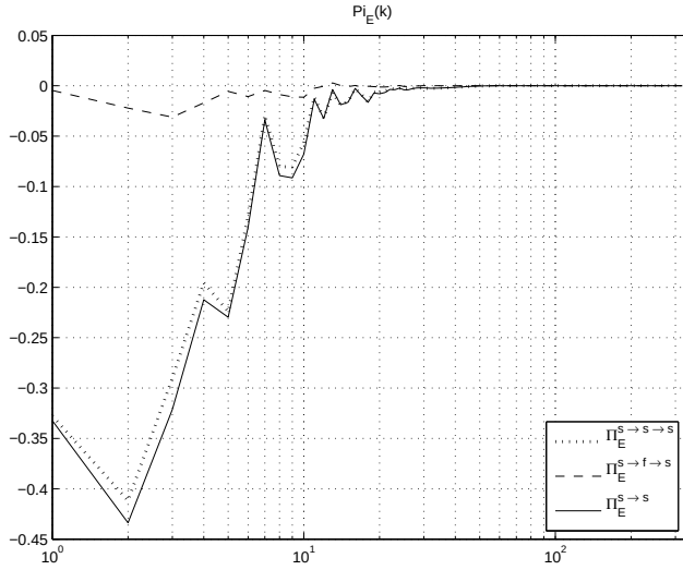
FIGURE 16. Decomposition of the main term responsible for the energy cascade ( k_{inj} \approx 20 ).
