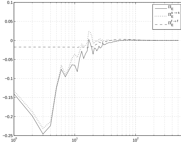
FIGURE 11. Energy fluxes of the whole flow and of the separate structures ( k_{inj} \approx 40 ).
