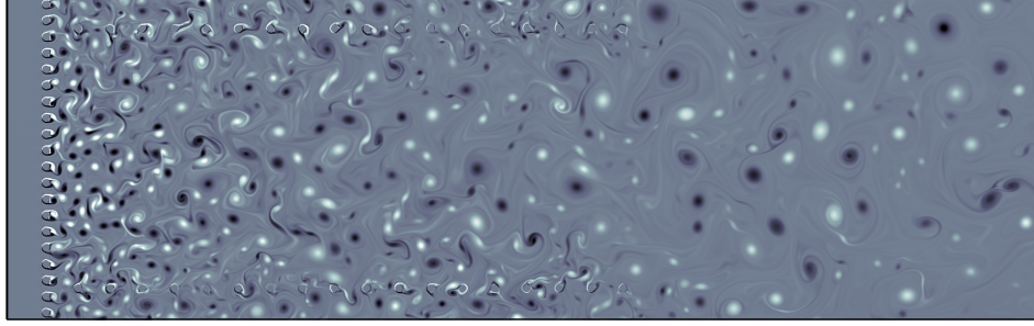
FIGURE 10. Snapshot of the vorticity field
