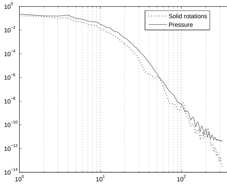
FIGURE 5. Pressure and solid rotations spectra ( k_{inj} \approx 20 ).
