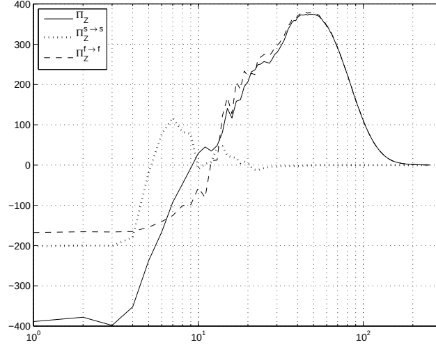
FIGURE 15. Enstrophy fluxes of the whole flow and of the separate structures ( k_{inj} \approx 9 ).
