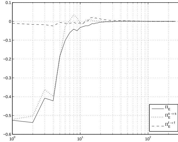
FIGURE 14. Energy fluxes of the whole flow and of the separate structures ( k_{inj} \approx 9 ).
