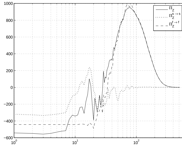
FIGURE 12. Enstrophy fluxes of the whole flow and of the separate structures ( k_{inj} \approx 40 ).
