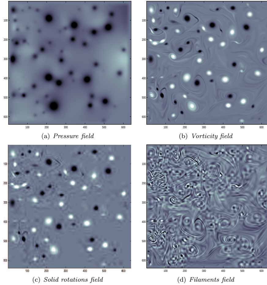
FIGURE 4. Snapshots at the end of the channel ( k_{inj} \approx 20 )
