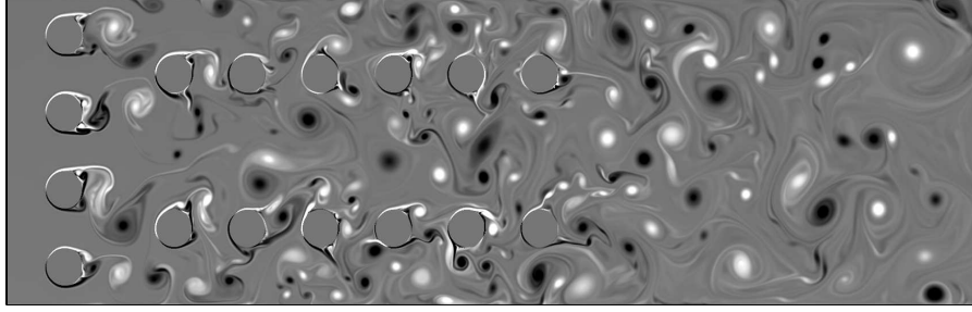
FIGURE 13. Snapshot of the vorticity field
