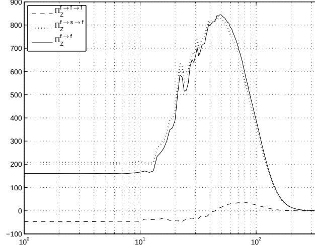
FIGURE 17. Decomposition of the main term responsible for the enstrophy cascade ( k_{inj} \approx 20 ).
