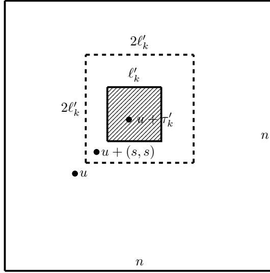
Fig. 1. The biggest square is the square pattern p \in \widetilde{\mathcal{A}}^{\llbracket 0, n \rrbracket^2} . Let u \in I(p, \ell'_k) . The dashed square of size 2\ell'_k is a pattern in \mathcal{L}(\widetilde{X}, 2\ell'_k) . The pattern located in the innermost square of size \ell'_k belongs to \widetilde{A}'_k \sqcup \widetilde{B}'_k . The innermost dot represents u + \tau'_k .
