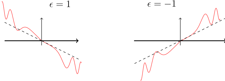
Fig. 2. Type II: On the left hand side, a growth at \pm\infty at least negative. On the right hand side, a growth at \pm\infty at least positive
