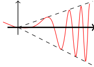
Fig. 5. The limits inferior and superior of linear growth at +\infty (or at -\infty ) have different signs
