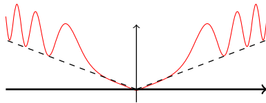
Fig. 6. At least negative (resp. positive) linear growth at -\infty (resp. +\infty ). The symmetric case with respect to the horizontal axis is also impossible
