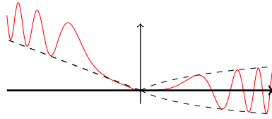
Fig. 4. At least (negative) linear growth at -\infty and sublinear growth at +\infty . The symmetric case with respect to the vertical axis is also impossible
