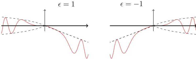
Fig. 3. On the left hand side, a sublinear growth at -\infty and a growth at +\infty at least negative. On the right hand side, a sublinear growth at +\infty and a growth at -\infty at least positive
