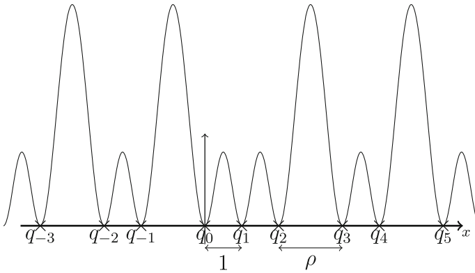
Fig. 7. Graph of the potential V for \alpha = 1/\sqrt{5} and \rho = \sqrt{3}
