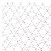
Figure 11.1.11 The Ammann bars of Figure 11.1.10 after the tiles have been deleted. The solid bars are to be regarded as the edges of a new tiling by rhombs and parallelograms, the dashed bars are to be regarded as markings on the tiles specifying the matching condition.
