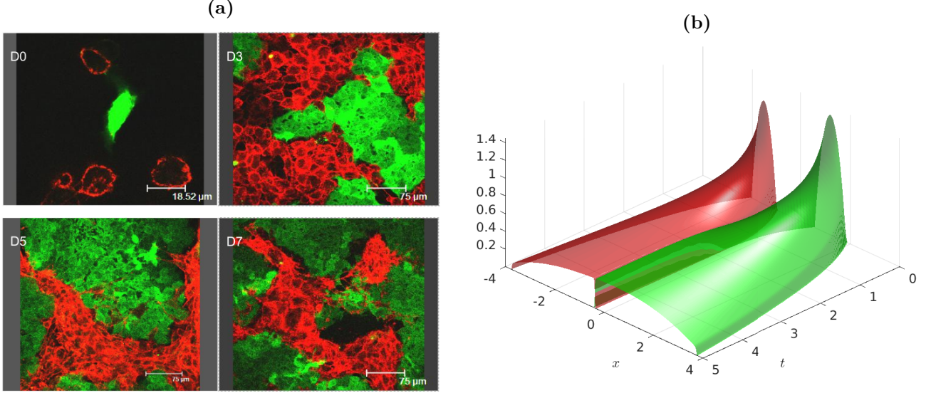
Figure 1: [23, Figure 1 and Figure 5 (b)]. (a) Direct immunodetection of P-gp transfers in co-cultures of sensitive (MCF-7) and resistant (MCF-7/Doxo) variants of the human breast cancer cell line. (b) The temporal-spatial evolution of the two species in the 1D model. One can check that a discontinuity is forming near the front face of the green surface.
