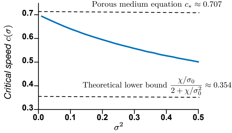
Figure 9: The relationship between parameter \sigma^2 and the critical propagation speed c(\sigma) by numerical simulations. Concerning the computation for the critical speed c , we take the speed on three level sets t \rightarrow \xi(t, \beta) + L for \beta = 0.3, 0.5, 0.8 and we plot the mean value (the standard variation is negligible \approx 10^{-3} ). As the critical speed c(\sigma) is decreasing with respect to \sigma , the theoretical lower bound is obtained by setting \chi = 1, \sigma_0 = 0.5 in Theorem 2.7.
