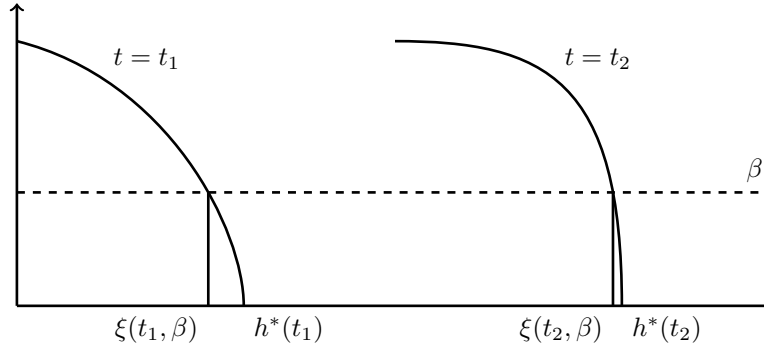
Figure 3: A cartoon for the formation of the discontinuity. Here we choose t_1 < t_2 and \xi(t, \beta), t = t_1, t_2 are the level sets. Theorem 2.5 proves that when Assumptions 2.1 and 2.2 are satisfied, then the distance |\xi(t, \beta) - h^*(t)| converges to 0 exponentially fast.
