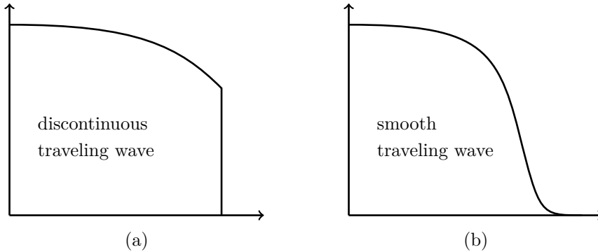
Figure 2: An illustration of two types of traveling wave solutions.
