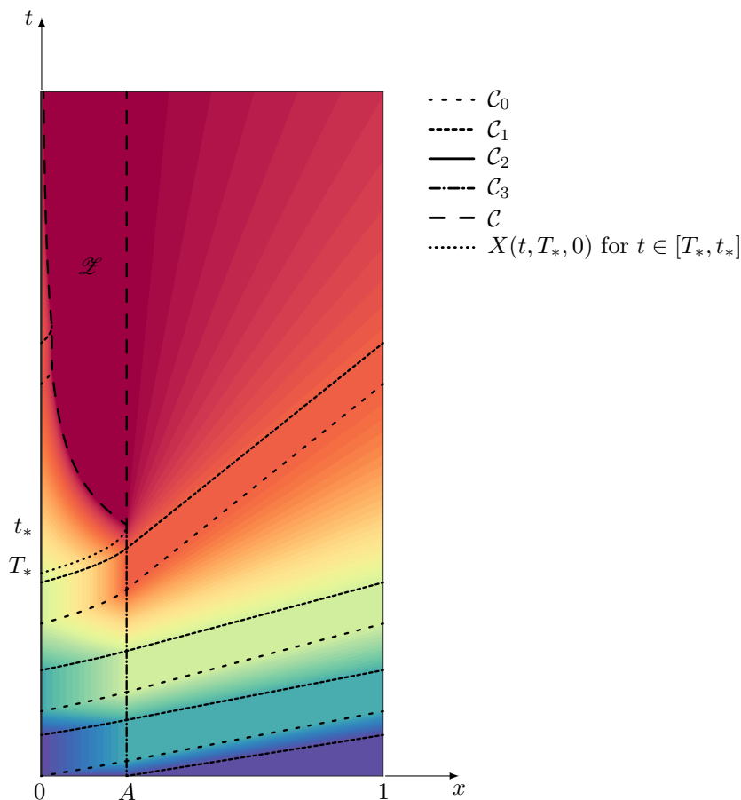
FIGURE 5.2. Discontinuity curves, \mathcal{Z} region and times T_* and t_* .
