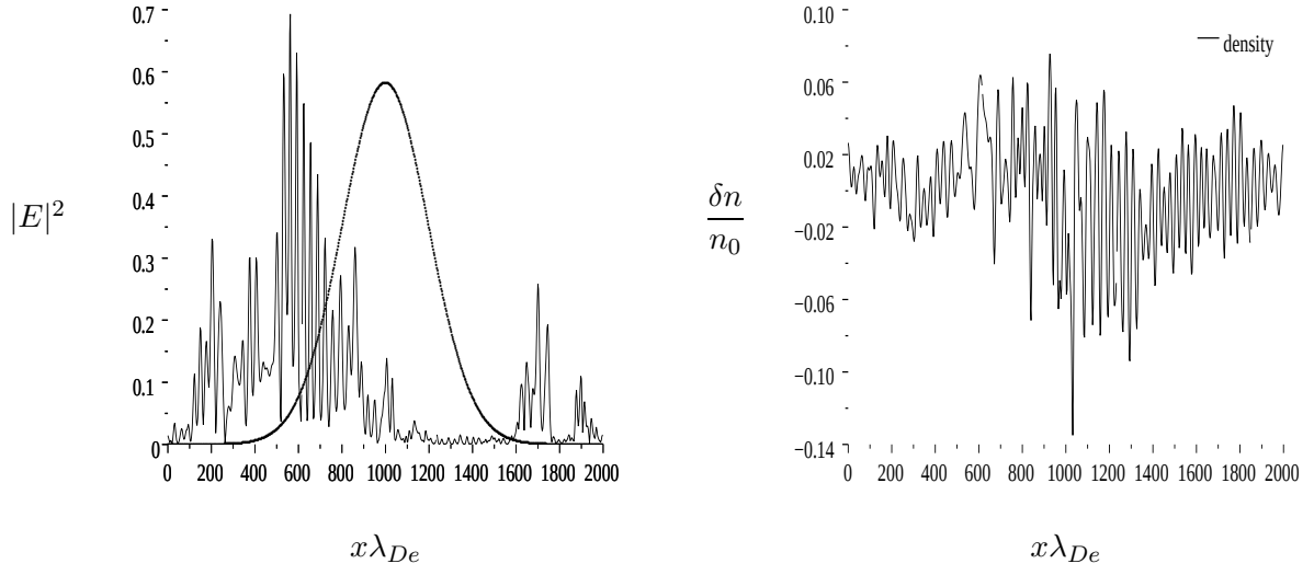
Figure 5: The left plot corresponds to the Langmuir wave in real space and the right plot corresponds to the low frequency density in real space
