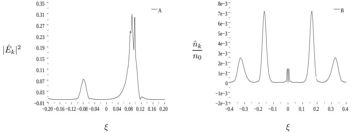
Figure 6: (A) corresponds to the Langmuir envelope spectra and (B) corresponds to the ion-acoustic spectra at the beginning of nonlinear processes.
