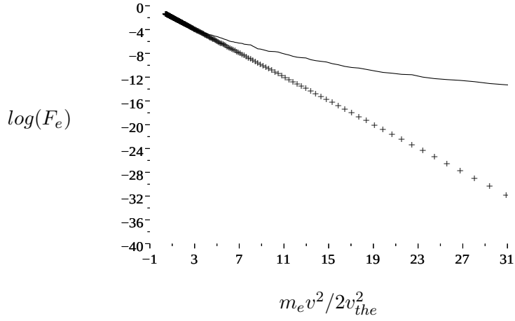
Figure 4: The solid line corresponds to the Log of the spatially averaged electron distribution versus the electron energy m_e v^2 / 2 v_{the}^2 at the final time \omega_{pe} t = 16000 with |S|/\sqrt{4\pi n_0 T_e} = 8.10^{-3} and k_p \lambda_{De} = 0.09 and the dashed line corresponds to the initial electron distribution.
