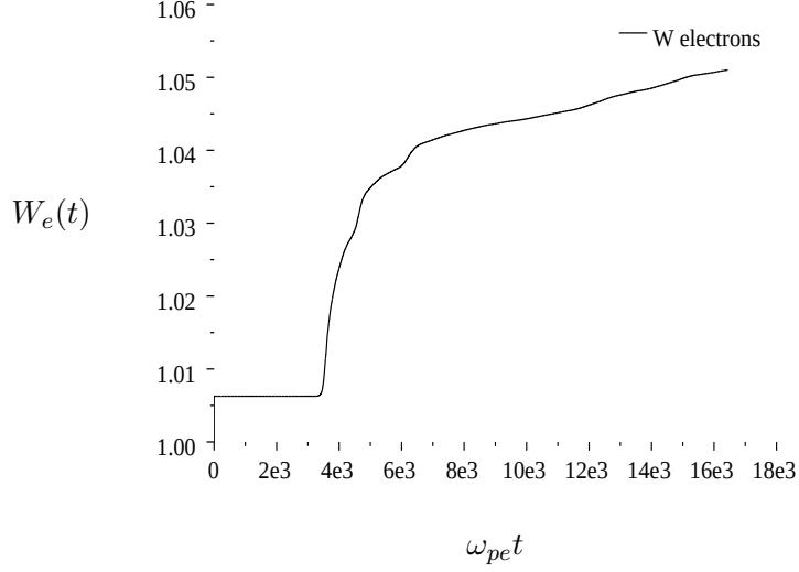
Figure 3: The time history W_e(t) of electron energy with |E_p| = 8.10^{-3} and k_1 \lambda_{De} = 0.09 .
