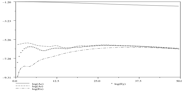
Figure 2. Neperian logarithm of the fiels with A_C(0) = 0.3e^{-0.01(y-35)^2}e^{-0.03(x-30)^2} , \frac{\omega_1}{\omega_0} = 0.01561
