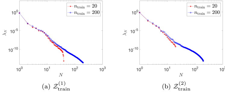
Fig. 3: Flow past a backstep: behavior of the POD modes for two datasets.
