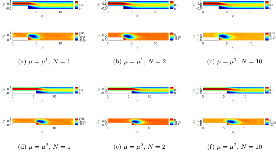
Fig. 7: Flow past a backstep: visualisation of the predicted field for three values of N and n_{\text{train}} = 200 . \mu^1 = [87.0307, 5.7174, 1.5635, 14.5669] , \mu^2 = [74.2651, 3.2926, 1.6392, 12.7344] .
