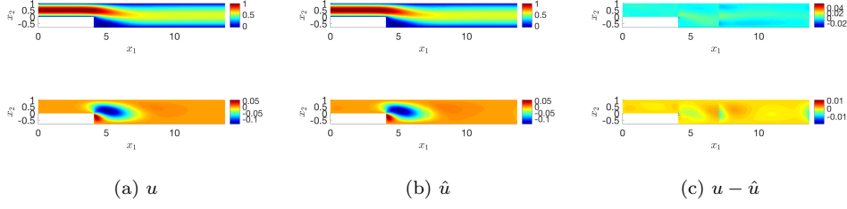
Fig. 9: Flow past a backstep: visualisation of the true and predicted fields for \mu = [59.59, 4.08, 1.78, 13.71] ( n_{\text{train}} = 200 ), here N = 10 .
