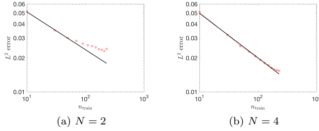
Fig. 10: Flow past a backstep: behavior of the relative mean L^2 error with n_{\text{train}} for N = 2 and N = 4 . The black trend lines correspond to the curves y(n) = 0.111n^{-0.335} for N = 2 , and y(n) = 0.124n^{-0.396} for N = 4 .
