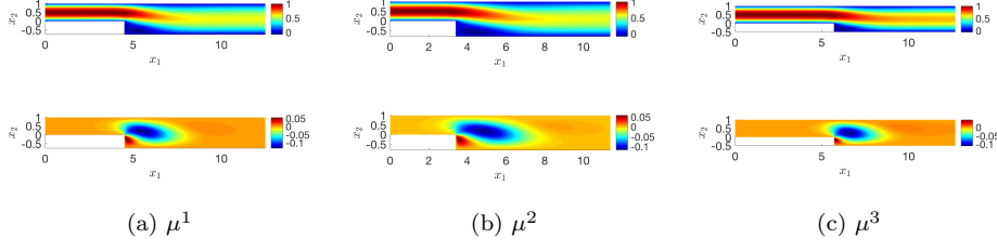
Fig. 2: Flow past a backstep: solution for three values of \mu \in \mathcal{P} : \mu^1 = [65, 4.5, 1.75, 12.5] , \mu^2 = [87, 3.4, 1.8, 11.4] , \mu^3 = [93, 5.7, 1.5, 12.7] .
