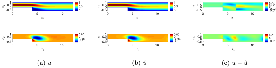
Fig. 8: Flow past a backstep: visualisation of the true and predicted fields for \mu = [71.82, 4, 1.65, 12.26] ( n_{\text{train}} = 200 ), here N = 10 .
