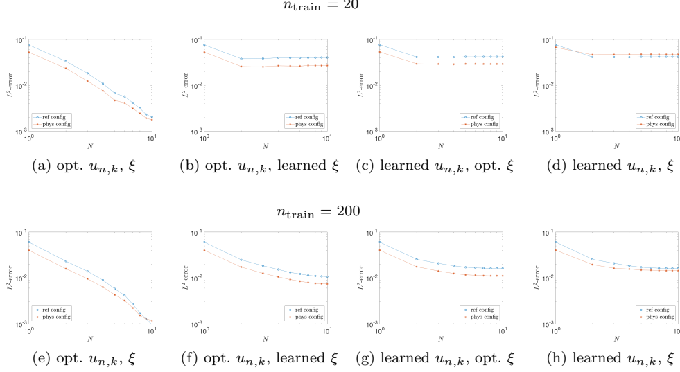
Fig. 6: Flow past a backstep: behavior of the mean relative L^2 error for n_{\text{test}} = 10 datapoints for optimal and learned expansion coefficients \{u_{n,k}\} and mapping parameter \xi , for two values of n_{\text{train}} .
