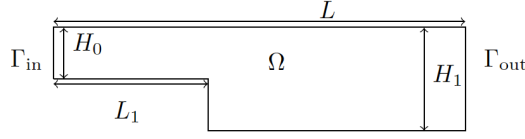
Fig. 1: Laminar flow past a backstep: computational domain.
