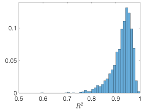
Fig. 4: Flow past a backstep: histogram of the out-of-sample coefficient of determination ( R^2 ) based on B 0.9-0.1 random split of the dataset ( B = 2000 , n_{\text{train}} = 200 ). The averaged R^2 is equal to 0.93.
