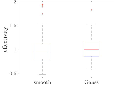
Figure 5: linear problem. Effectivity of the error indicator \eta = \frac{\hat{E}(n_{\text{test}}=10)}{\hat{E}(n_{\text{test}}=100)} for 100 independent runs and for both Gaussian and smooth training.
